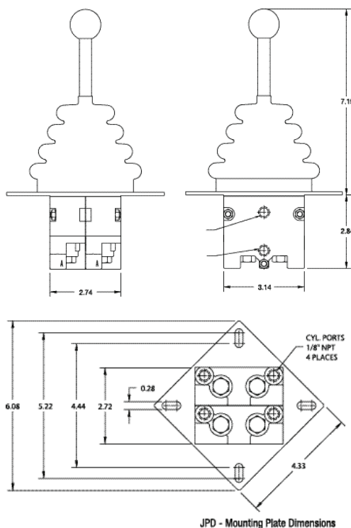
JPD - Mounting Plate Dimensions
