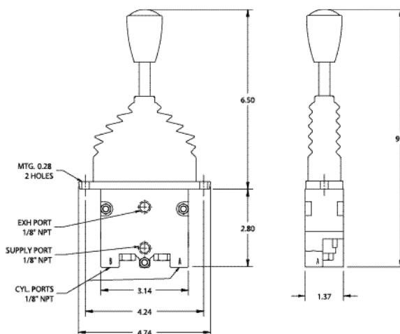
JPD - Mounting Plate Dimensions
